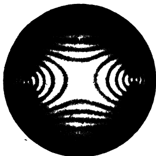
FIG. 57.—Appearance of the Interference Figure half a Minute after commencing the Experiment. Temperature of Crystal about 40^{\circ} C.
